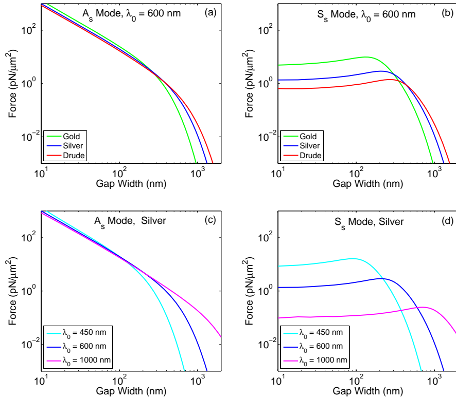
Fig. 7. (a) and (b): The force from the SPP modes in the IMIMI geometry, calculated using three models for the metal: tabulated data for gold (green lines) and silver (blue lines), and the Drude Model (red lines) at an operating wavelength of \lambda_0 = 600\text{nm} . Plotted in (a) is the magnitude of the attractive A_s mode force, while the repulsive S_s mode force is plotted in (b). (c) and (d): The A_s and S_s mode forces between silver slabs at \lambda_0 = 450\text{nm} (cyan lines), \lambda_0 = 600\text{nm} (blue lines), \lambda_0 = 1000\text{nm} (magenta lines). The MIM A_0 mode behaves like the IMIMI A_s mode, and so is not plotted here.
