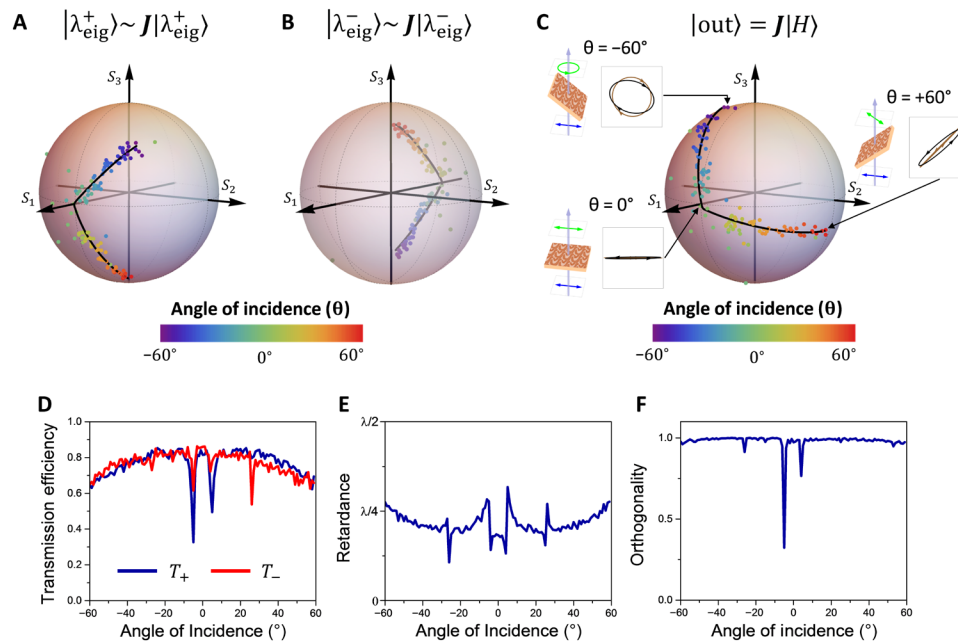
Fig. 4. Measurement results for a continuous angular range. (A and B) Measured eigen-polarization states |\lambda_{\text{eig}}^{\pm}\rangle at various angles of incidence. The color represents the angle of incidence ( \theta ). Both the ellipticity and the orientation, which is related to the latitude and longitude of the Poincaré sphere, respectively (fig. S7), of the eigen-polarization states vary significantly as a function of the angle of incidence. The solid black line is a fitted curve of the trajectory. (C) Measured output polarization states ( |\text{out}\rangle ) for a fixed incident polarization state |H\rangle . As \theta angle changes from -60^\circ to 60^\circ , the output polarization state follows a nonconventional trajectory on the Poincaré sphere, which goes continuously from nearly right circular polarization ( S_3 ) through horizontal linear polarization ( S_1 ) to nearly 45^\circ linear polarization ( S_2 ). The schematic, as well as the measured (black) and simulated (brown) polarization ellipses at 0^\circ and \pm 60^\circ , are highlighted in the insets. (D) Measured transmission efficiency for the two eigen-polarization states |\lambda_{\text{eig}}^+ (blue line) and |\lambda_{\text{eig}}^- (red line). The transmission dips result from excitation of guided mode resonances. (E) Measured retardance. (F) Measured orthogonality of the two eigen-polarization states. It is defined as 1 - |\langle \lambda_{\text{eig}}^+ | \lambda_{\text{eig}}^- \rangle|^2 . Away from the resonances, the two eigenstates are almost orthogonal.
