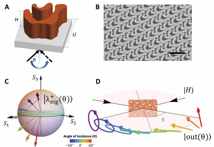
Fig. 2. Topology-optimized structure element. (A) Schematic of the optimized structure. It consists of freeform amorphous silicon (a-Si) nanostructures patterned on top of a glass substrate. The a-Si thickness is H = 1500 nm. The center-to-center distance between neighboring elements is U = 600 nm. (B) SEM image of a fabricated sample. Scale bar, 1 \mu\text{m} . (C) The arrows represent the angle-dependent eigen-polarization states ( |\lambda_{\text{eig}}^{\pm}(\theta)\rangle ) of the device. Different colors correspond to different angles of incidence ( \theta ). As one varies the angle, the device can be continuously tuned between linear and elliptical birefringence. (D) Angle-dependent polarization generation. For a fixed incident polarization ( |in\rangle = |H\rangle ), the output polarization state ( |out(\theta)\rangle = J(\theta)|H\rangle ) changes continuously from right circular polarization through horizontal linear polarization to 45^\circ linear polarization for varying angle of incidence.
