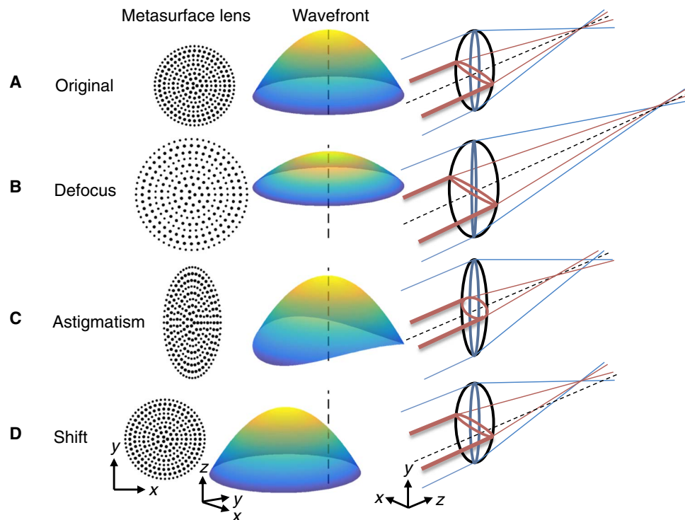
Fig. 1. Principle of strain field-mediated tunable metalens. A metasurface (left column) is constructed by digitizing an analog optical phase profile on a flat surface into discrete cells, each of which contains a metasurface element that locally imparts the required phase shift to the incident light to reconstruct the desired wavefront (middle column; dashed line: optical axis). The wavefront generated by the metasurface determines the subsequent beam shaping (right column). (A) Original: metasurface without stretch. (B) Defocus: metasurface with uniform and isotropic stretch. (C) Astigmatism: metasurface under asymmetric stretch. (D) Shift: metasurface displaced laterally in the x,y plane.
