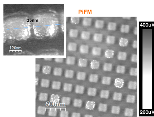
Figure 3. PiFM image of the TiO 2 squares embedded in ZEP photoresist. The PiFM signal is the amplitude from the lock-in amplifier demodulating at the first eigenmode frequency \omega_0 . The second eigenmode of the cantilever is instead used to retrieve the sample morphology and for tip-to-sample distance stabilization. The two materials have different refractive indices and are almost completely transparent to the illuminating light. Here the material with higher refractive index produces the lower PiFM signal. The figure's inset shows the PiFM image of a gap of 35 nm between two TiO 2 squared structures.
