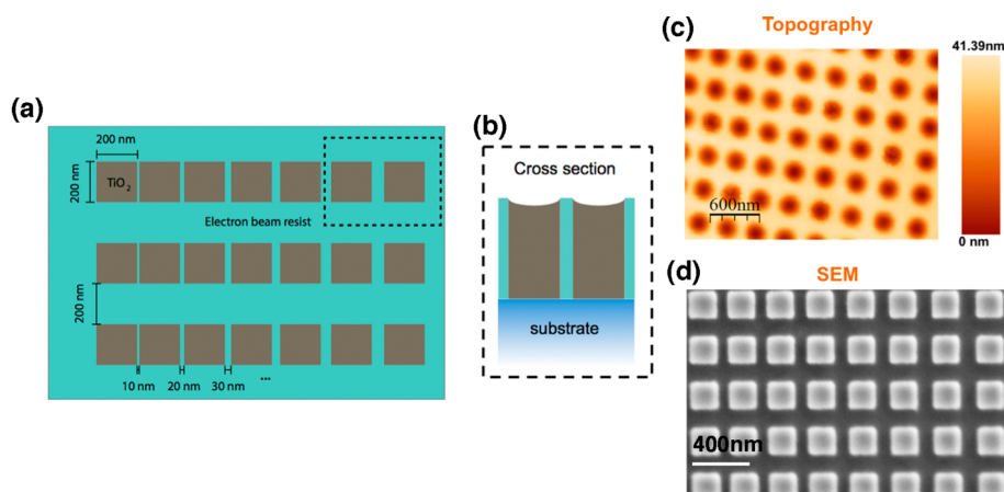
Figure 2. (a) Sample consists of an array of titanium dioxide (TiO 2 ) squares embedded in a matrix of electron beam resist (ZEP 520A, ZEON Corp.) on a fused silica substrate. In one direction, the array consists of 21 individual TiO 2 squares with an increasing gap between each successive square. In the orthogonal direction the TiO 2 squares are offset from each other by a constant distance. (b) Cross section of the TiO 2 structures. The sample is typically overetched by nominal 10–20 nm. This results into shallow hemispherical troughs in the surface morphology clearly seen in AFM topography (c). (d) SEM micrographs of the same sample showing the TiO 2 squares embedded in the ZEP matrix. From the SEM image, the TiO 2 squares are 230 nm × 230 nm, with 170 nm space between two rows.
