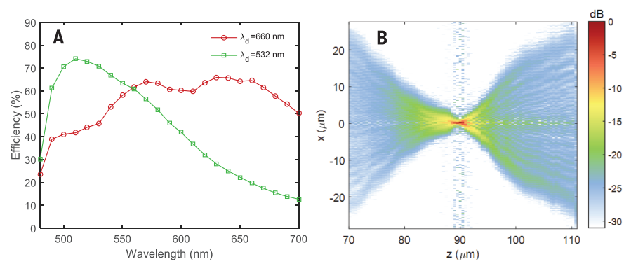
Fig. 3. Characterization of the metalenses. (A) Measured focusing efficiency of the metalenses designed at wavelengths of 660 nm and 532 nm. (B) Intensity distribution in dB of the x-z plane, showing the evolution of the beam from 20 \mu\text{m} before and 20 \mu\text{m} after the focus. This measurement was performed on the metalens designed at \lambda_d = 532 nm. The wavelength of incident light was 532 nm.
