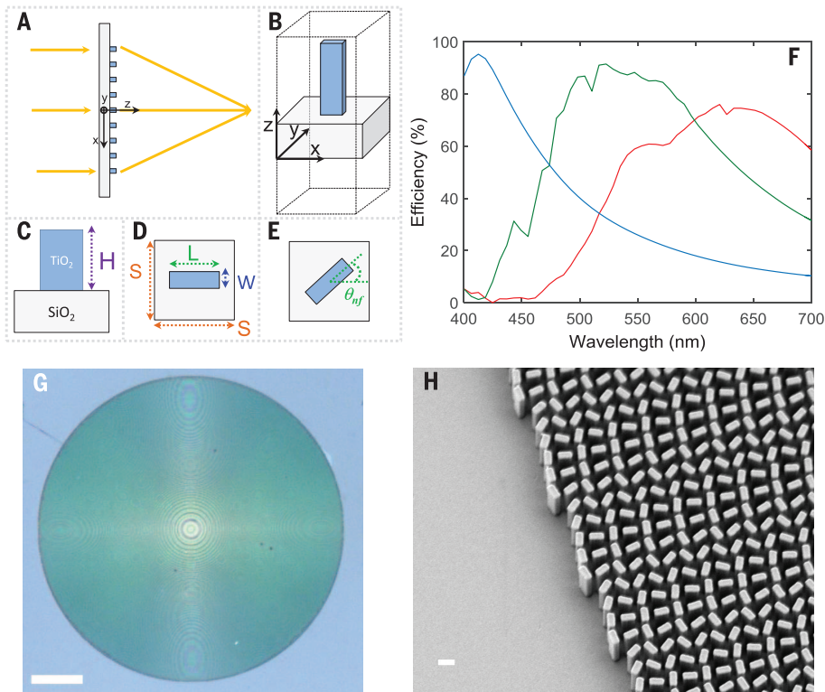
Fig. 1. Design and fabrication of metalenses. (A) Schematic of the metalens and its building block, the TiO 2 nanofin. (B) The metalens consists of TiO 2 nanofins on a glass substrate. (C and D) Side and top views of the unit cell showing height H , width W , and length L of the nanofin, with unit cell dimensions S \times S . (E) The required phase is imparted by rotation of the nanofin by an angle \theta_{nf} , according to the geometric Pancharatnam-Berry phase. (F) Simulated polarization conversion efficiency as a function of wavelength. This efficiency is defined as the fraction of the incident circularly polarized optical power that is converted to transmitted optical power with opposite helicity. For these simulations, periodic boundary conditions are applied at the x and y boundaries and perfectly matched layers at the z boundaries. For the metalens designed at \lambda_d = 660 nm (red curve), nanofins have W = 85 , L = 410 , and H = 600 nm, with center-to-center spacing S = 430 nm. For the metalens designed at \lambda_d = 532 nm (green curve), nanofins have W = 95 , L = 250 , and H = 600 nm, with center-to-center spacing S = 325 nm. For the metalens designed at \lambda_d = 405 nm (blue curve), nanofins have W = 40 , L = 150 , and H = 600 nm, with center-to-center spacing S = 200 nm. (G) Optical image of the metalens designed at the wavelength of 660 nm. Scale bar, 40 \mu\text{m} . (H) SEM micrograph of the fabricated metalens. Scale bar, 300 nm.
