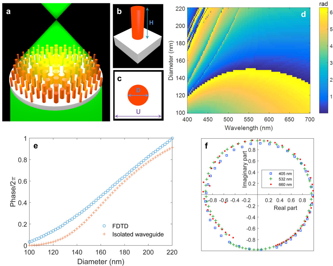
Figure 1. (a) Schematic of a metalens operating in transmission mode. (b,c) Side-view and top-view of the metalens building block: a \text{TiO}_2 nanopillar on a glass substrate. Here we arranged nanopillars in a square lattice. For the design wavelength \lambda_d = 405 nm ( \lambda_d = 532 nm; \lambda_d = 660 nm), the unit cell dimension is U = 180 nm ( U = 250 nm; U = 350 nm), the nanopillar height is H = 400 nm ( H = 600 nm; H = 600 nm), and the nanopillar diameters D vary between 80 to 155 nm ( 100 nm < D < 220 nm; 100 nm < D < 320 nm). (d) Simulated phase map \phi(D) for the metalens designed at \lambda_d = 532 nm. Each point on this phase map shows the relative phase difference between a nanopillar with diameter D and a reference point where there is no nanopillar (propagation through the air). (e) Comparison of the phase calculated by finite difference time domain simulation of the building block (nanopillar on a glass substrate) as a function of diameter D , and the phase due to propagation in an isolated cylindrical waveguide, considering just its fundamental mode HE_{11} at \lambda_d = 532 nm. (f) Complex transmission coefficients for three design wavelengths. Each point represents the amplitude and phase of the transmission of a nanopillar with diameter D .
