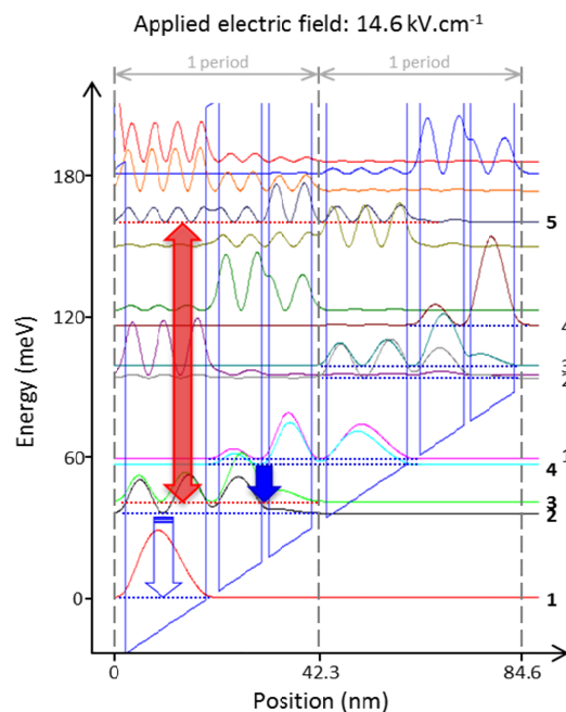
Figure 1 - Schematic bandstructure diagram showing coherent enhancement of the gain in a THz QCL. Arrows: terahertz laser transition (blue); LO-phonon emission (white); mid-infrared pump (red)
