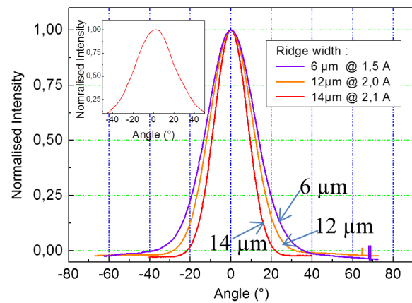
Fig. 8 Far-field pattern of the buried lasers with different ridge widths of 6 to 14 μm showing TM_{00} behavior. The main frame is the far field with respect to the slow axis and the inset is the far field with respect to the fast axis. Only one far field is shown in the fast axis since it is not influenced by the ridge width.
