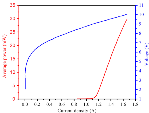
Fig. 3 I-V-L curve of BH-QCL emitting at 5.5 \mu\text{m} measured at 20°C under pulsed conditions (duty cycle –5%, repetition rate –20 kHz). 3-mm-long chips with 17.5- \mu\text{m} -wide ridges were mounted epi-side up on copper heat sink.
