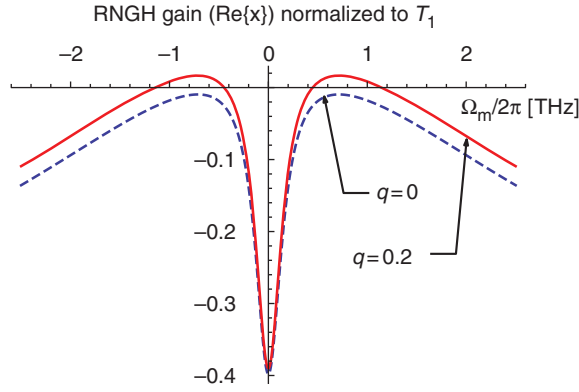
Figure 9. Growth rate of the R NGH instability, defined as a real part of x in Equation (27), as a function of the mode frequency for d=2 and two values of the normalized unsaturated losses in the absorber: q=0 (dashed curve) and q=0.2 (solid curve). The instability takes place where \Re\{x\} > 0 . (The color version of this figure is included in the online version of the journal.)
