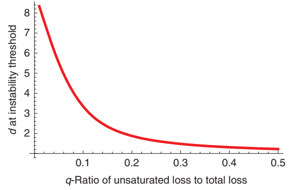
Figure 10. Pumping parameter d corresponding to R NGH instability threshold normalized to pumping at CW lasing threshold as a function of the unsaturated loss in the absorber q normalized to the total photon losses in the cavity. (The color version of this figure is included in the online version of the journal.)
