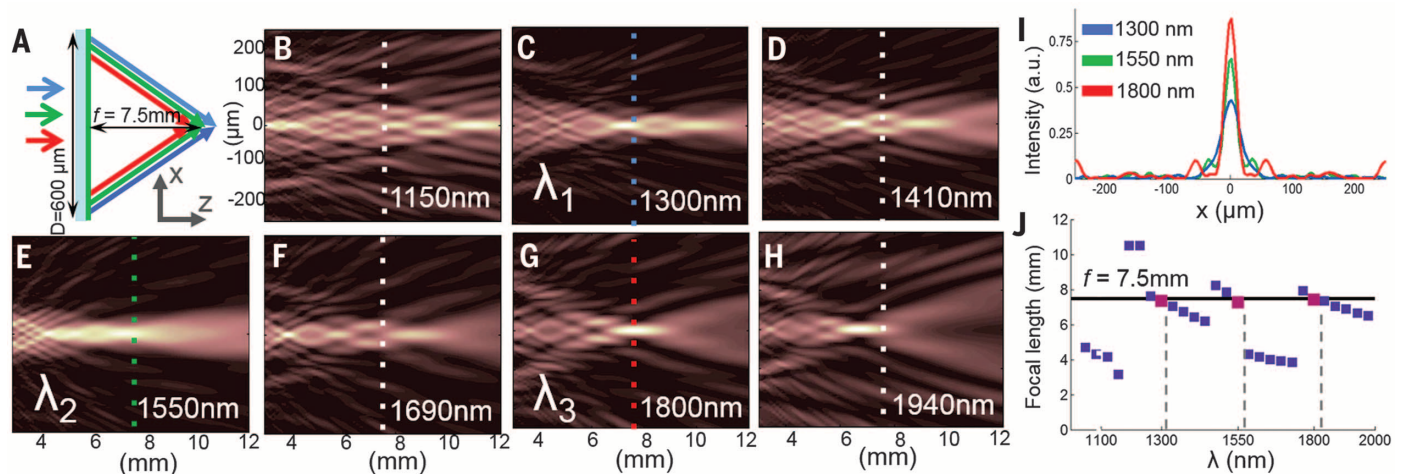
Fig. 4. Performance of a simulated achromatic flat lens. (A) A broadband plane wave illuminates the backside of the lens with side D = 600 \mu\text{m} and focal distance f = 7.5 \text{ mm} . (B to H) Far-field intensity distribution for different wavelengths. The dashed lines correspond to the desired focal planes. (I) Cross section across the focal plane for \lambda_1 , \lambda_2 , and \lambda_3 . (J) Focal lengths as a function of wavelength, calculated as the distance between the lens center and highest-intensity point on the optical axis. The three pink squares correspond to the wavelengths of interest.
