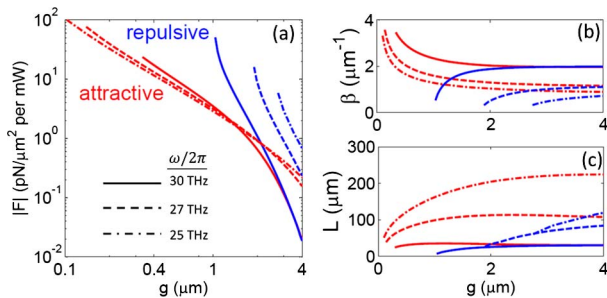
Fig. 3. (a) Attractive (red lines) and repulsive (blue lines) forces generated by the bonding and antibonding modes, respectively, at three wavelengths: \omega/2\pi = 30 \text{ THz} (solid lines), 27 THz (dashed lines), and 25 THz (dashed-dotted lines), as a function of gap width. (b) Wavevectors of these modes showing degeneracy at large gaps and splitting at small gaps. The antibonding mode has a clear cutoff gap. (c) Propagation length of the bonding (red) and antibonding (blue) modes plotted in (a).
