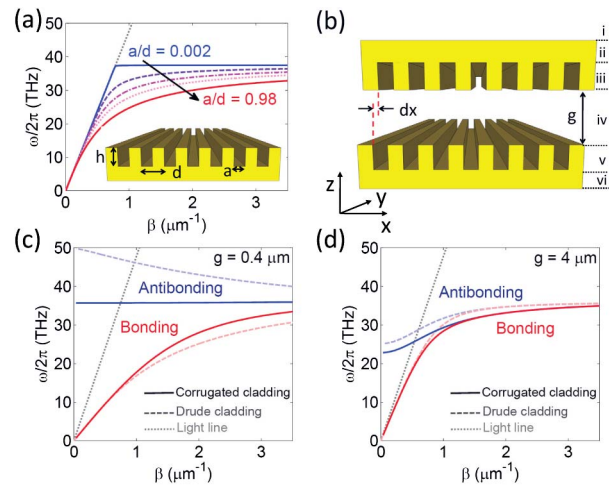
Fig. 1. (a) Dispersion relation of a single SSP mode, Eq. (1), for h = 2 \mu\text{m} , d = 0.5 \mu\text{m} , and a/d = [0.002, 0.2, 0.4, 0.6, 0.98] (solid-blue to solid-red line), where h , d , and a are defined in the inset. The black arrow represents increasing a/d . (b) Spoof-insulator-spoof (SIS) waveguide geometry consisting of a corrugated PEC cladding surrounding an air-gap core. Roman numerals I–VI correspond to the layers of the waveguide for dispersion calculations. (c), (d) Bonding (red) and antibonding (blue) modes in a SIS waveguide for (c) g = 0.4 \mu\text{m} (d) and g = 4 \mu\text{m} . For comparison, the modes of an MIM waveguide consisting of artificial Drude metals with plasma frequency \omega_p = \sqrt{2}\omega_{\text{ssp},0} are plotted as faded dashed lines in (c) and (d). The light line (gray-dotted line) is included for clarity.
